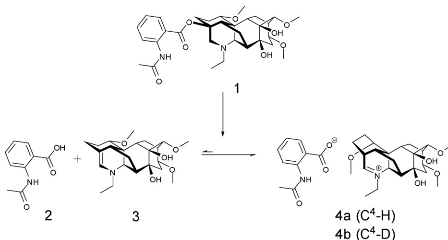
Scheme 1. Photo-induced decomposition of lappaconitine in solution.
